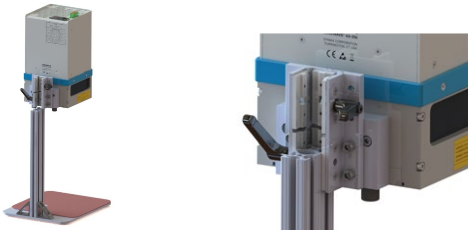
Figure 3. Slide Carriage into Stand
