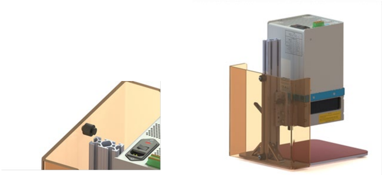
Figure 4. Slide Back Panel into Position
