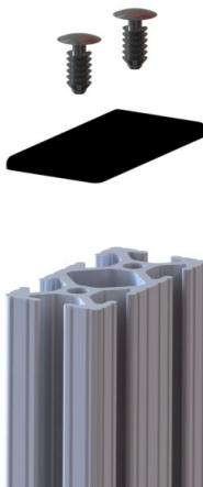
Figure 5. Cap and Fasteners
