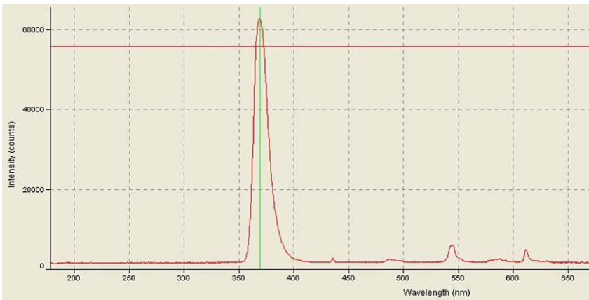
Figure 32. BlueWave LED Flood with RediCure Array – 365 nm Spectral Output
