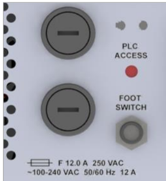
Figure 25. Fuse Holders
